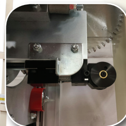
Scoring System
